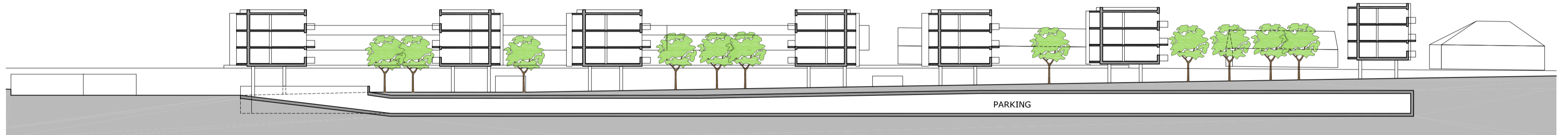
Section A 1:500
